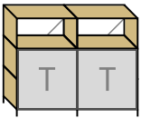
SC/M5-02 Size: 138 × 113 cm Depth: 53 cm Back: wood / open Door: 67,5 × 67,5 cm transparent
