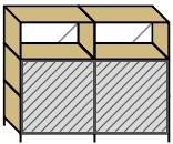
SC/M5-03 Size: 138 × 113 cm Depth: 53 cm Back: wood / open Door: 67,5 × 67,5 cm slash
