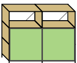
SC/M5-05 Size: 138 × 113 cm Depth: 53 cm Back: wood / open Door: 67,5 × 67,5 cm green
